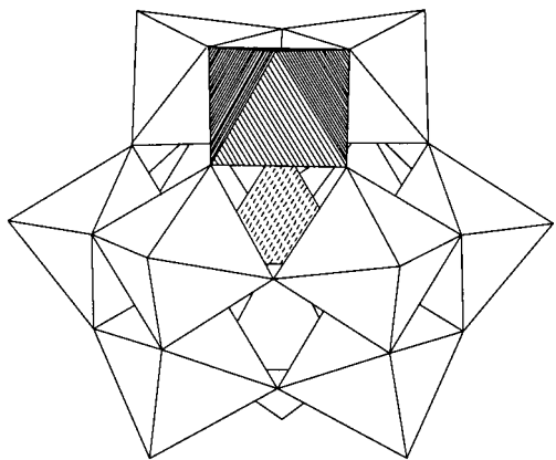
Figure 1. Drawing (in polyhedral notation) of \alpha -SiVW 11 O 40 5- ( 1 ) where the central tetrahedron represents the Si IV O 4 unit, the shaded octahedron represents V V O 6 , and the unshaded octahedra represent W V O 6 units.
