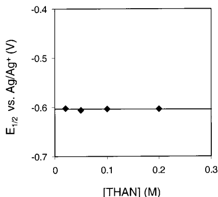
Figure 6. Potential, E_{1/2} , of the 1/I_{red} couple (1.0 mM THA_5I ) in 2:3 (v/v) H_2O/t -BuOH at 60 °C in the presence of 25–200 mM tetra- n -hexylammonium nitrate (THAN) electrolyte. E_{1/2} values are referenced to Ag/AgNO_3 (see Experimental Section).
