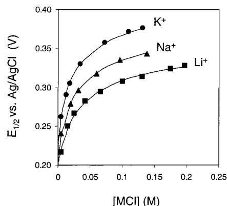
Figure 8. Plot of E_{1/2} versus [\text{M}^+] ( \text{M}^+ = \text{Li}^+, \text{Na}^+, \text{and K}^+ ); [\text{M}^+] = [\text{MCl}] + 5[\text{M}_5\mathbf{1}] + [\text{MOAc}] , [\text{MCl}] = 0.0\text{--}0.2 \text{ M} , [\text{M}_5\mathbf{1}] = 1.0 \text{ mM} , [\text{MOAc}] = 1 \text{ mM} , [\text{HOAc}] = 1 \text{ mM} , 60^\circ \text{C} , E_{1/2} versus Ag/AgCl electrode. (Solid curves are from nonlinear least-squares fitting of the data to eq 42.)
