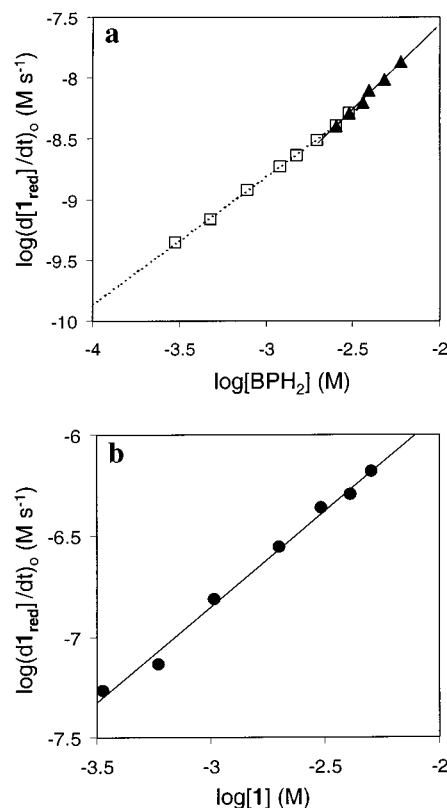
Figure 2. (a) Plot of \log(\text{initial rate} = d[\mathbf{1}_{\text{red}}]/dt) versus \log [\text{BPH}_2] ; [BPH 2 ] = 0.3–3.6 mM (dashed line, the slope is 1.06) and [BPH 2 ] = 3.0–6.0 mM (solid triangles), [Li 5 1] = 0.4 mM, [LiOAc] = 0.1 M, [HOAc] = 0.1 M, 60 °C. (b) Plot of \log(\text{initial rate} = d[\mathbf{1}_{\text{red}}]/dt) versus \log [\mathbf{1}] ; [Li 5 1] = 0.34–5.0 mM, [BPH 2 ] = 6.0 mM, [LiOAc] = 0.1 M, [HOAc] = 0.1 M, 60 °C.
