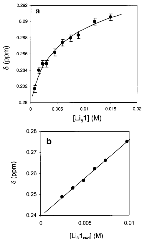
Figure 9. (a) Chemical shift of the 7 Li NMR signal (relative to 1.0 M LiCl in D 2 O) as the concentration of Li 5 1 is increased from 0.3 to 15 mM (1.5–75 mM Li + ) in 2:3 (v/v) H 2 O/ t -BuOH at 60 °C. A digital resolution of 0.061 Hz (0.0004 ppm) was used to accurately measure the relatively small changes in chemical shift values. Solid curve: nonlinear least-squares fit to eq 28 (see Experimental Section); \delta_0 = 0.287 ppm, \delta_1 = 0.336 ppm, K_{Li1} = 65 \pm 35 M -1 (95% confidence interval). (b) Chemical shift of the 7 Li NMR signal as the concentration of Li 6 1 red is increased from 0.5 to 10 mM in 2:3 (v/v) H 2 O/ t -BuOH at 60 °C. The slope ( \Delta\delta_{obs} M -1 ) is 3.62 ppm M -1 ( R^2 = 0.998 ).
