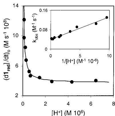
Figure 3. Plot of initial rate = d[\mathbf{I}_{\text{red}}]/dt versus [\text{H}^+] ; [\text{H}^+] = 6.5 \times 10^{-6} - 1.3 \times 10^{-7} (pH = 5.19–6.89 measured in acetate-buffered water/ t -BuOH), [\text{Li}_5\mathbf{1}] = 0.48 mM, [\text{BPH}_2] = 2.86 mM, [\text{LiOAc}] = 0.1 M, 60 °C. Inset: Plot of k_{\text{obs}} versus 1/[\text{H}^+] .
