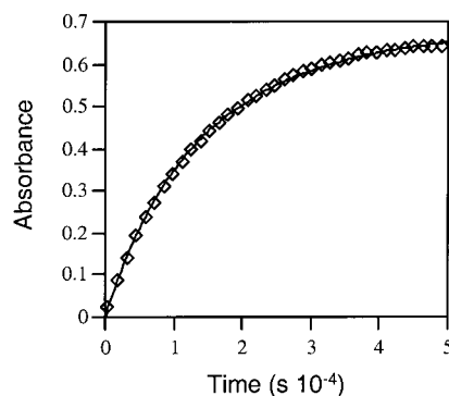
Figure 5. Absorbance at 520 nm ( I_{red} ) versus time data (open diamonds; for clarity, every other point is plotted) for the oxidation of BPH 2 by Li 5 1 and nonlinear least-squares fit of eq 37 (solid line; k_{obs} = 2.02 \times 10^{-2} \text{ M}^{-1} \text{ s}^{-1} , sum of standardized square residuals = 2.9 \times 10^{-3} ). Reaction conditions: [1] = 1.1 \text{ mM} , [BPH_2] = 1.9 \text{ mM} , [LiOAc] = 1 \text{ mM} , [HOAc] = 1 \text{ mM} , [LiCl] = 10.2 \text{ mM} , 2:3 (v/v) H 2 O/ t -BuOH, under Ar at 60 °C.
